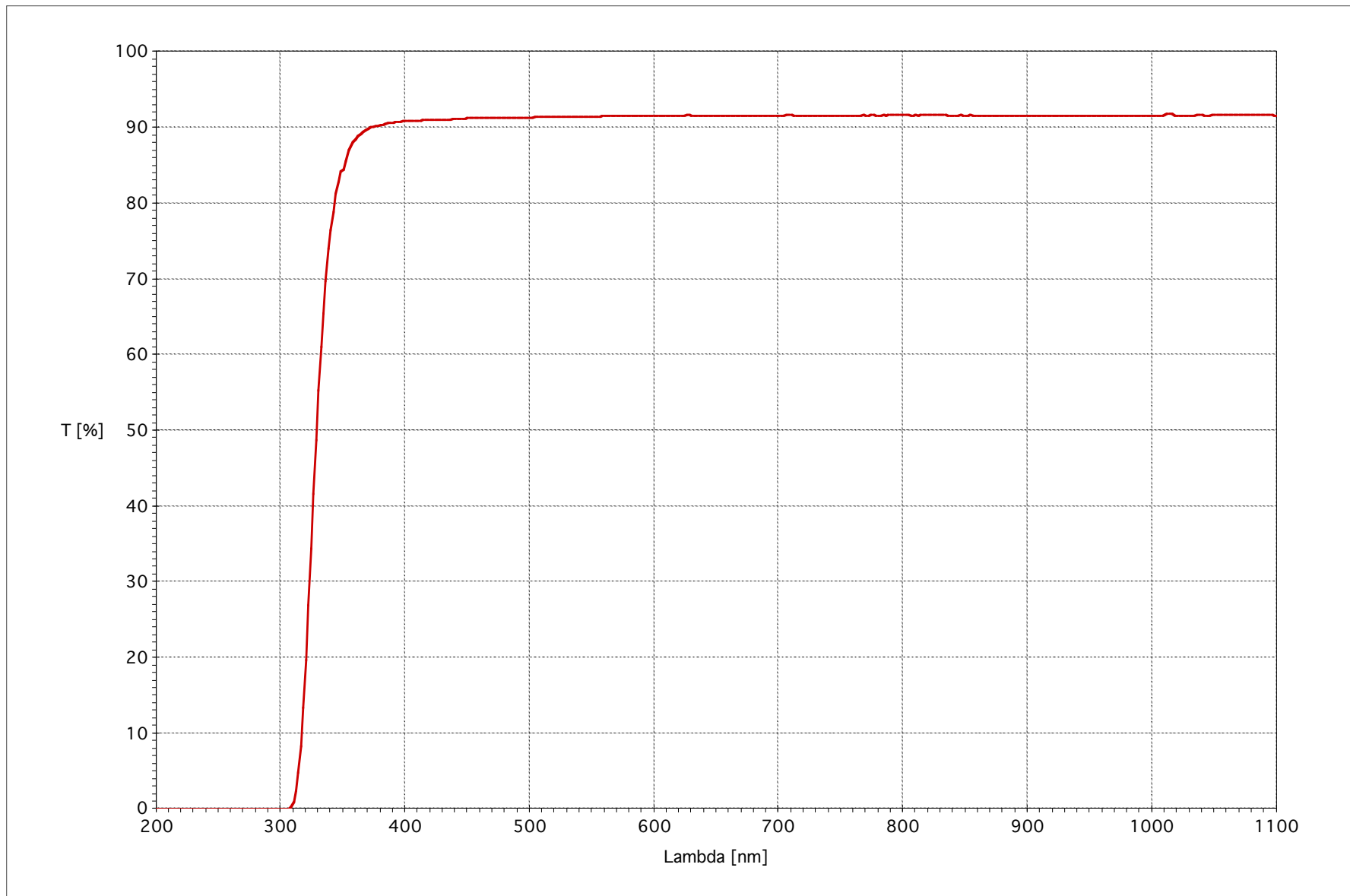
D263 Transmissionsspektrum, 200-1100nm, Substrate thickness: 0,7mm
