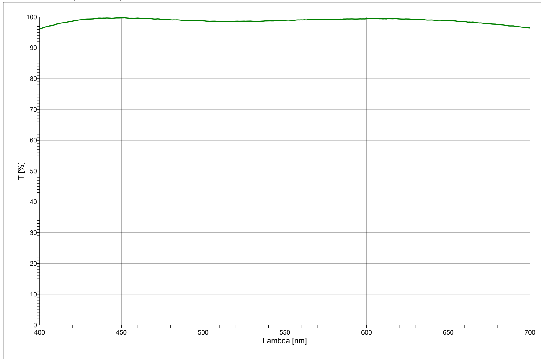
ARC-O Transmission, 400-700nm, Substrate thickness: 3mm
