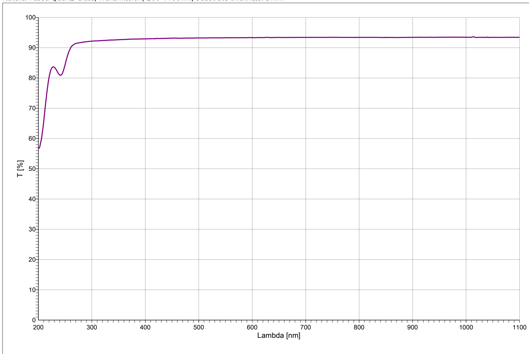
Natural Fused Quartz Glass, Transmission, 200-1100nm, Substrate thickness: 3mm
