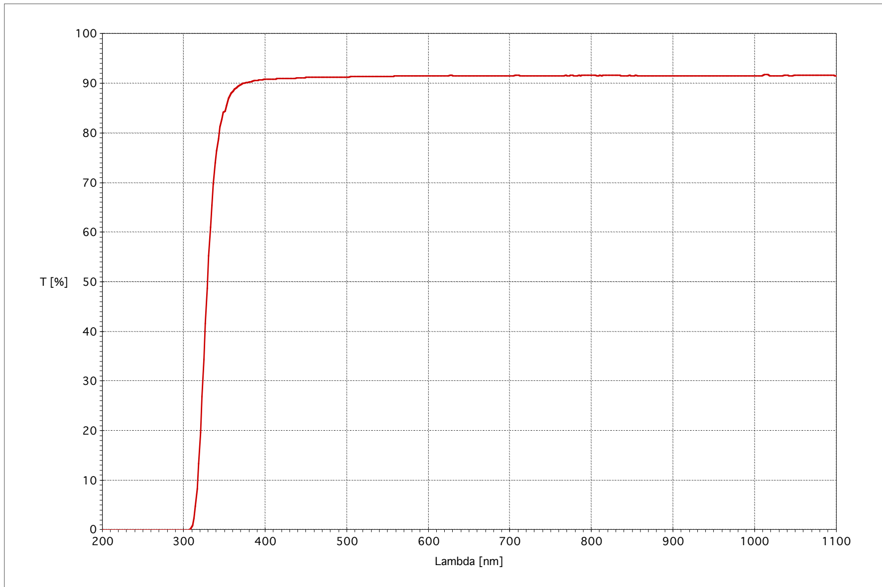
D263 Transmissionsspektrum, 200-1100nm, Substrate thickness: 0,7mm
