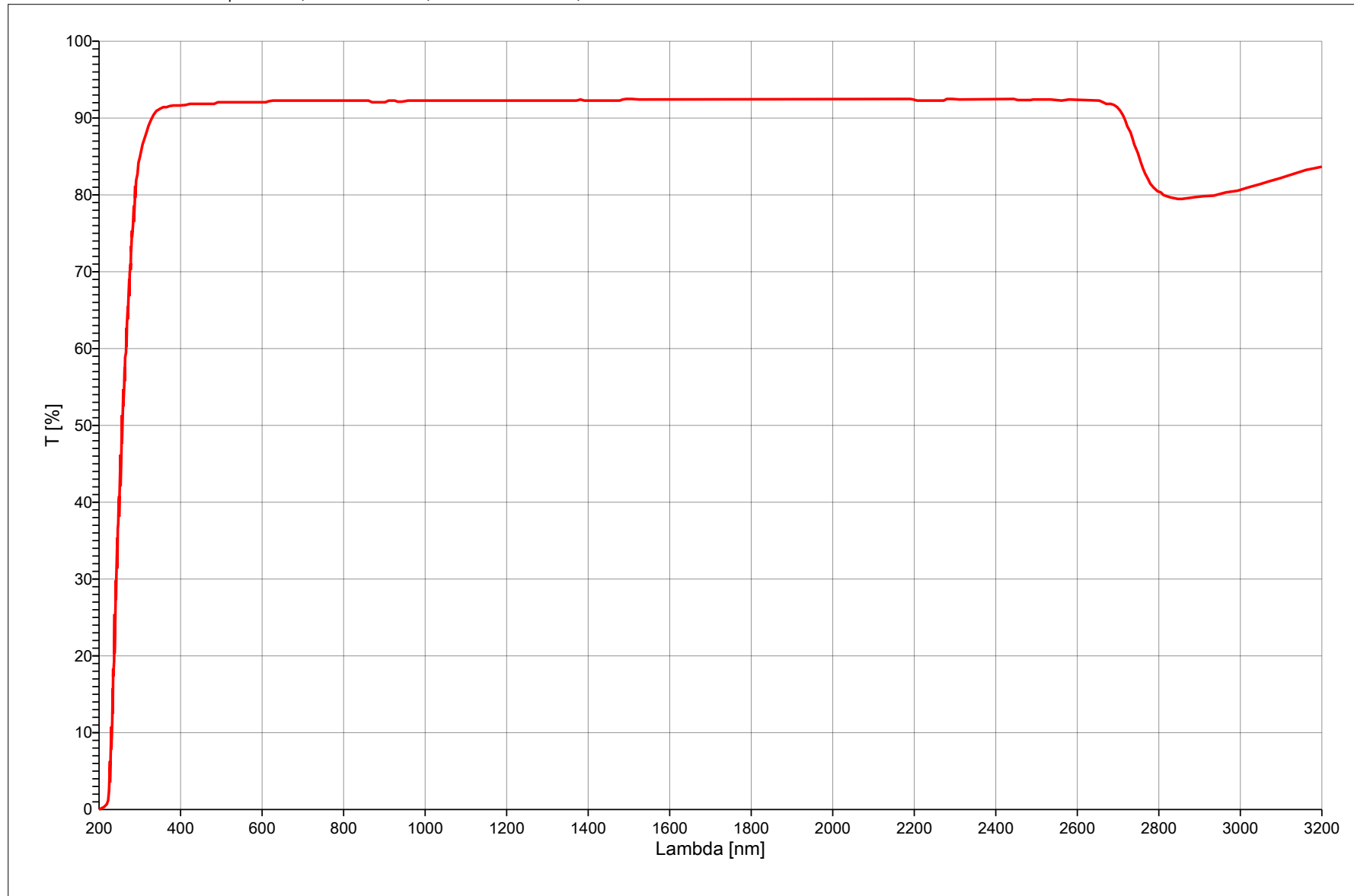
AS 87 eco Transmissionsspektrum, 200-3200nm, Substratdicke: 0,175mm
