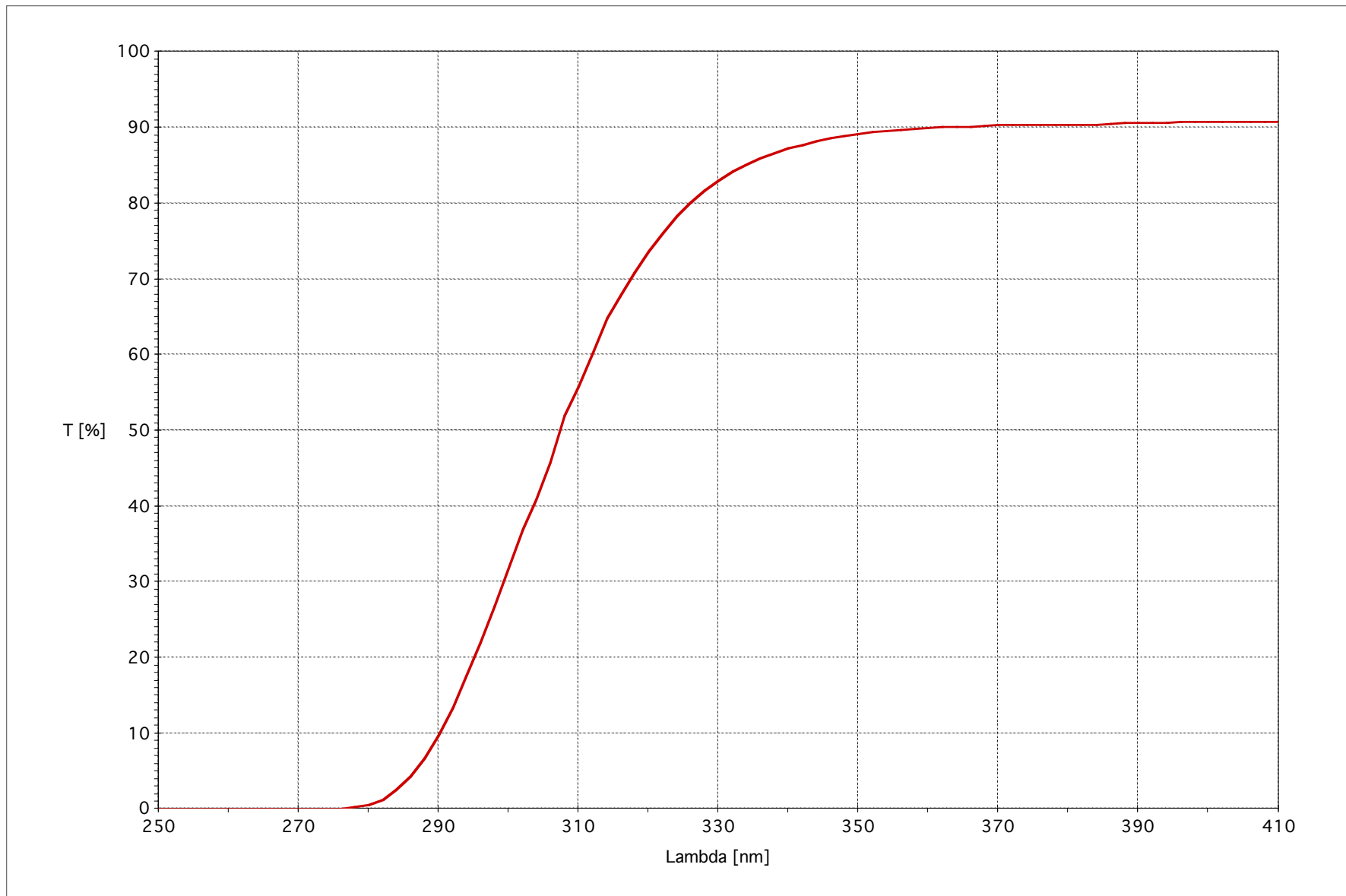
B270 UV-Transmission, 250-410nm, Substratdicke: 1,15mm
