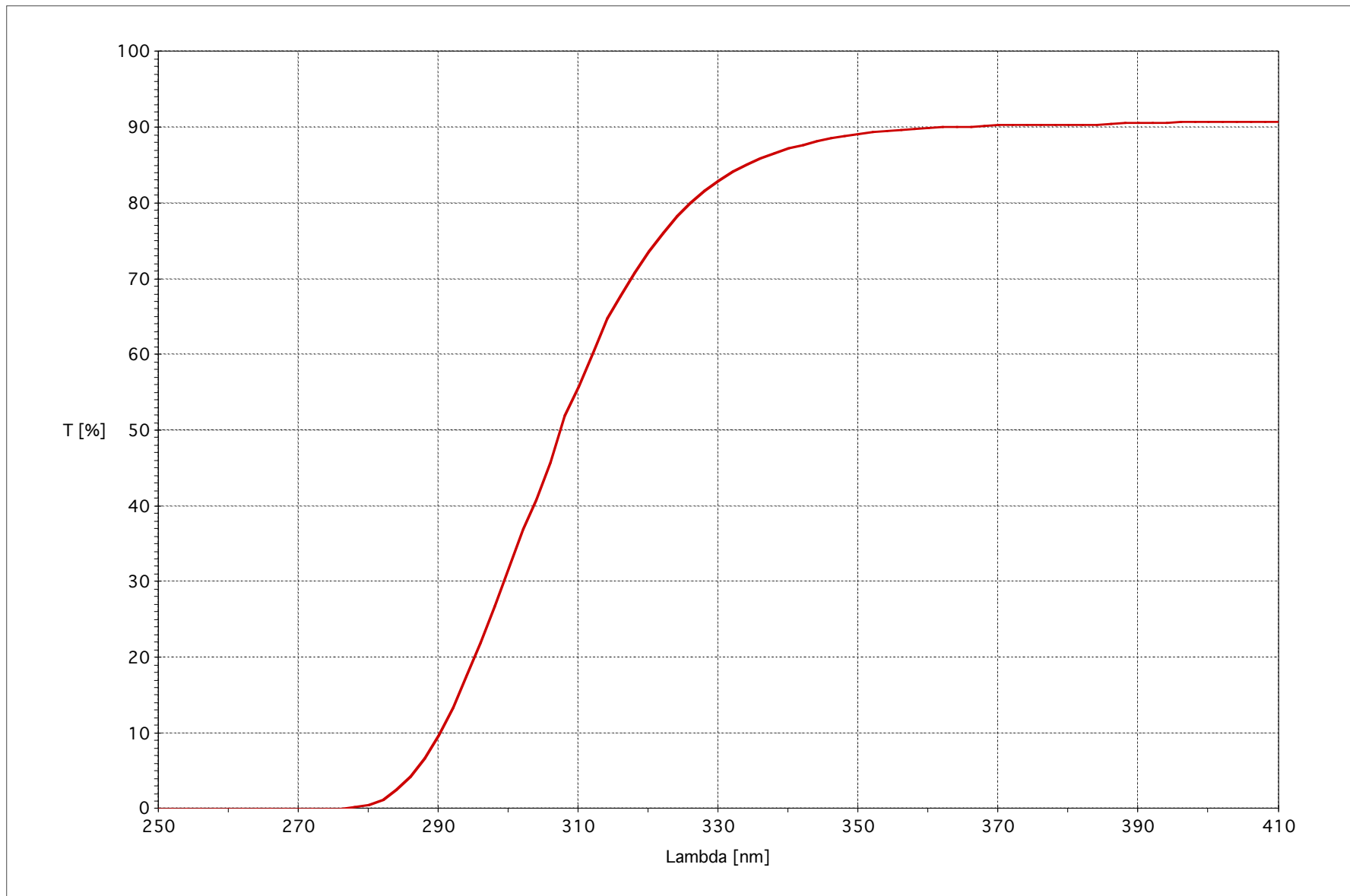
B270 UV-Transmission, 250-410nm, Substratdicke: 1,15mm
