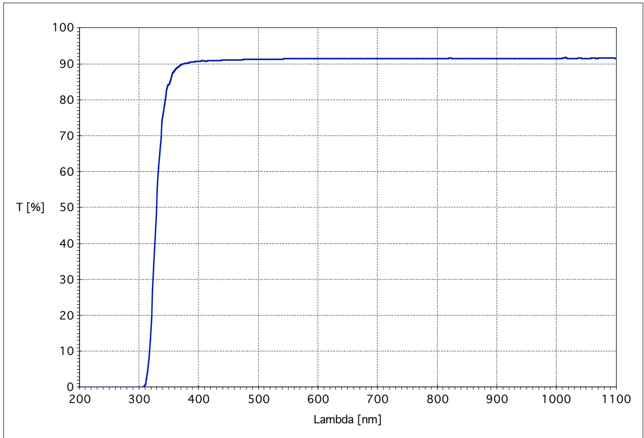
D263 T, Optical Transmission Spectrum, 200-1100nm, Substrate thickness: 0,7mm
